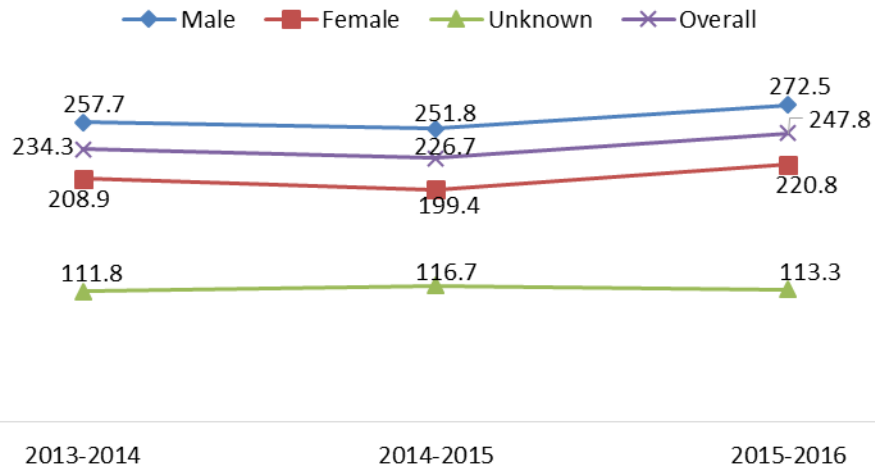
Figure 54: Average Number of Hours by Gender
