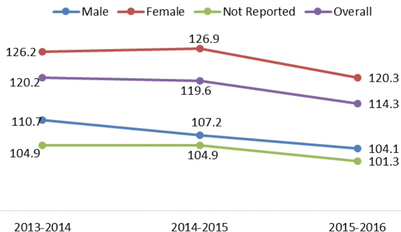
Figure 44: Average Number of Hours Completed by ESL Program by Gender
