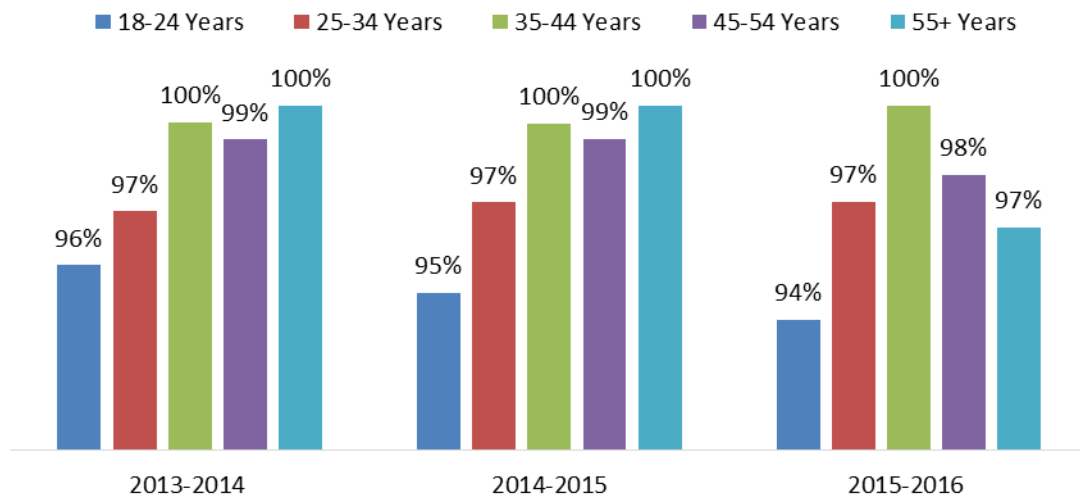
Figure 15: SCE High School/GED Program Success Rates by Age
